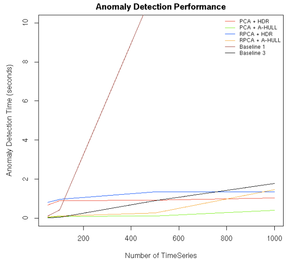
Fig. 4. Scalability performance
