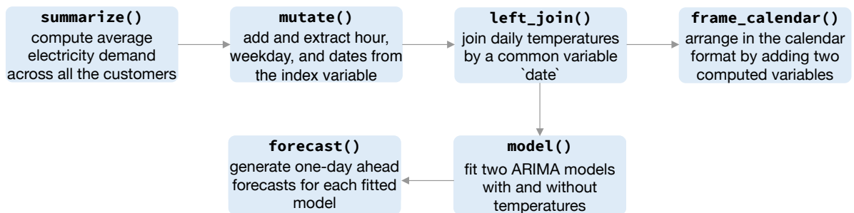
Figure 12: Flow chart illustrating the pipeline involved for creating Figure 10 and Figure 11.
