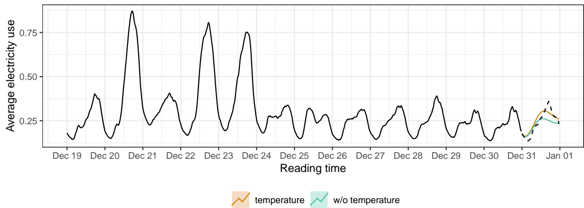
Figure 11: One-day (48 steps ahead) forecasts generated by ARIMA models, with and without a temperature covariate, plotted against the actual demand. Both nicely capture the temporal dynamics, but ARIMA with temperature performs better than the model without.
